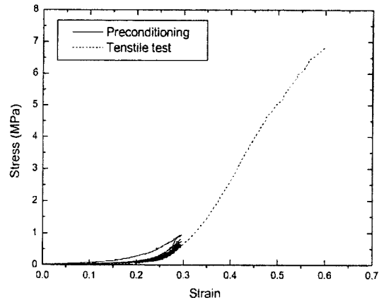
Fig. 9 Relationship between stress and strain of pig's leg vessels
